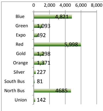
YTD Citations - 20208
