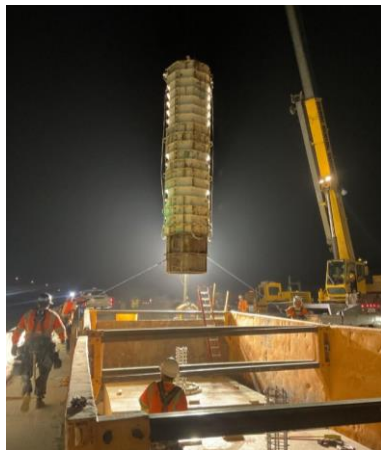
Erection of Column for new Weldon Canyon bridge
