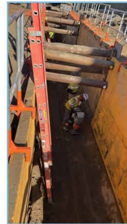
Preparing Base for Storm Drain at D5
