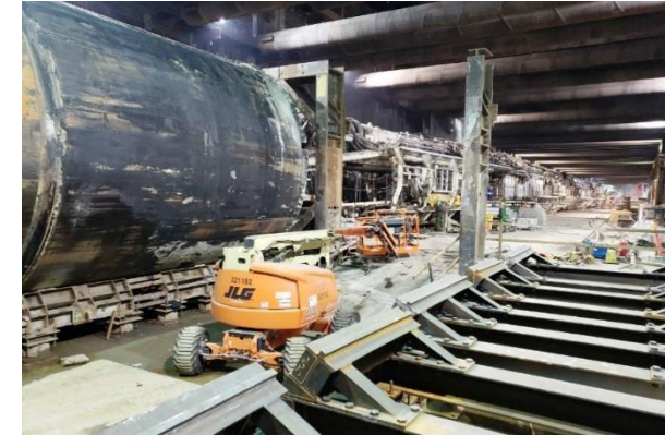
Purple TBM at Wilshire/Fairfax Station
